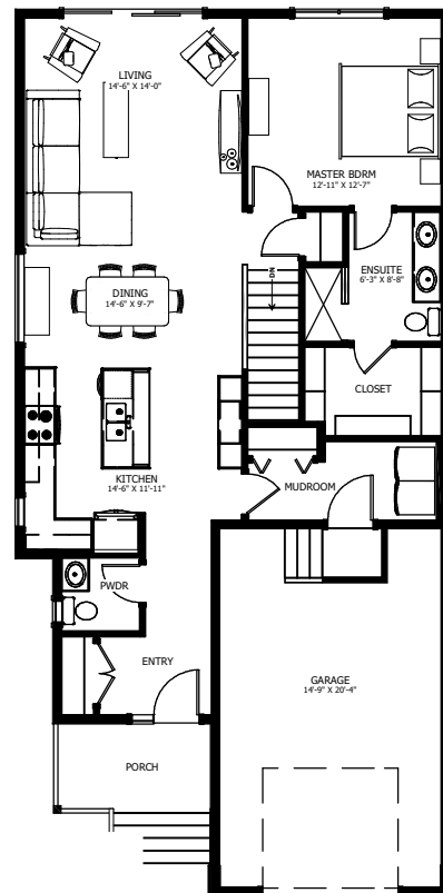
MAIN FLOOR PLAN LIVING AREA: 970 SQ.FT
